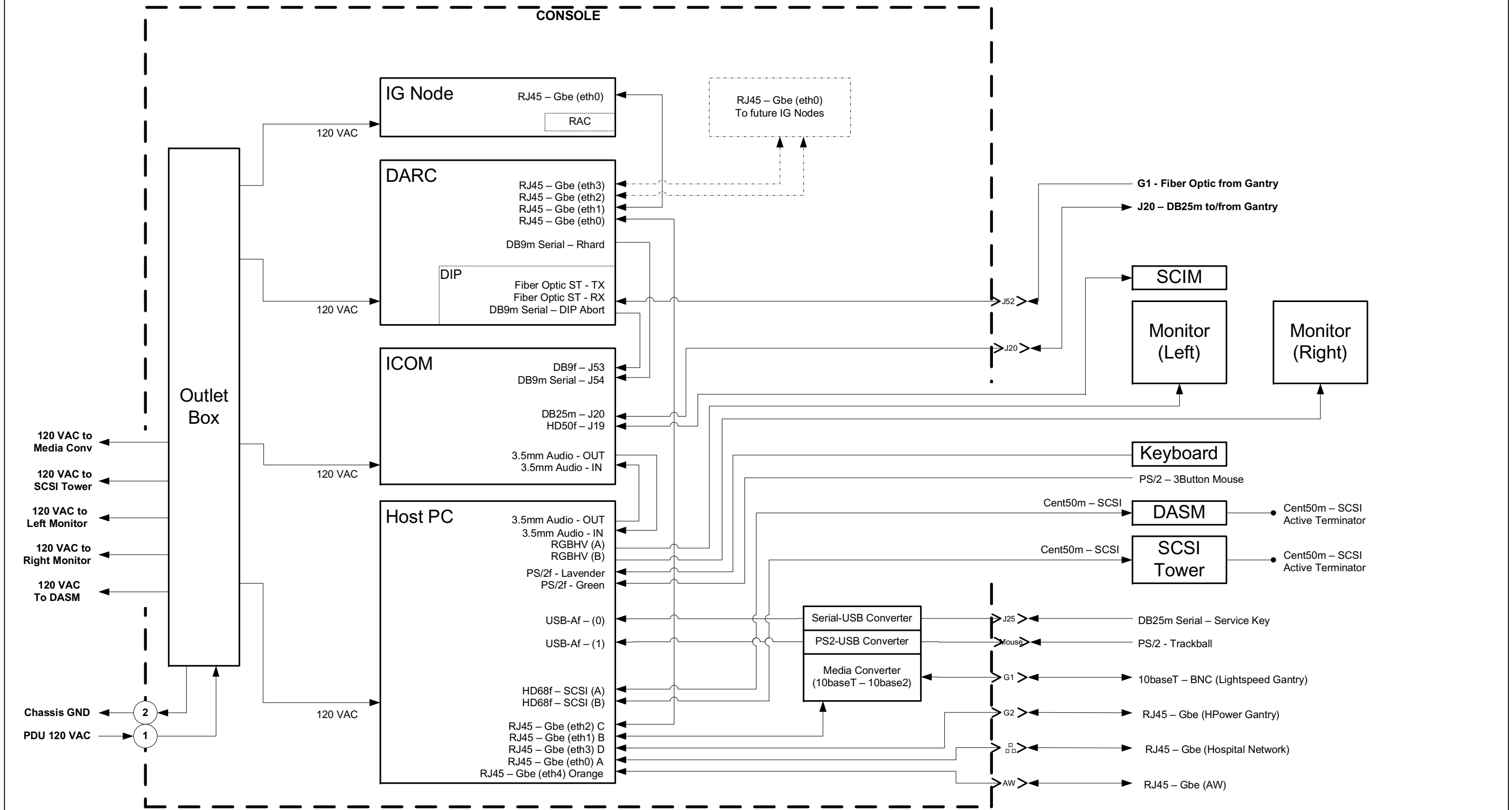
Console (GOC4/LCGOC) Block Diagram
